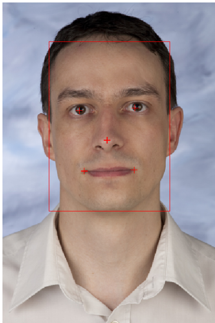
mtcnn
