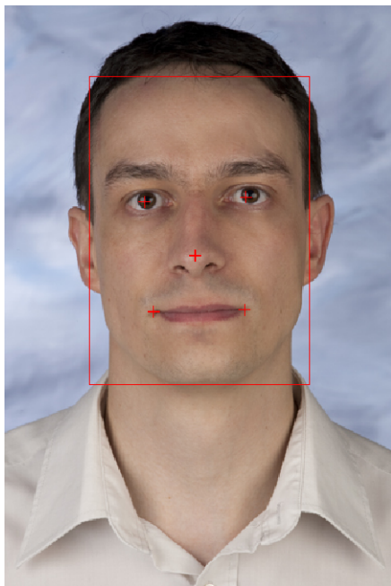
mtcnn
