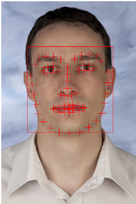
Dlib landmarks
