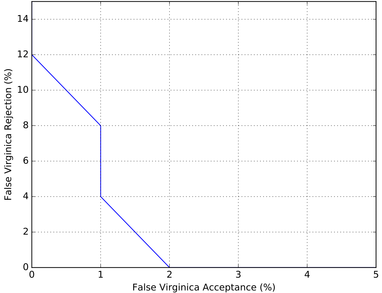
ROC Curve for Virginica Classification
