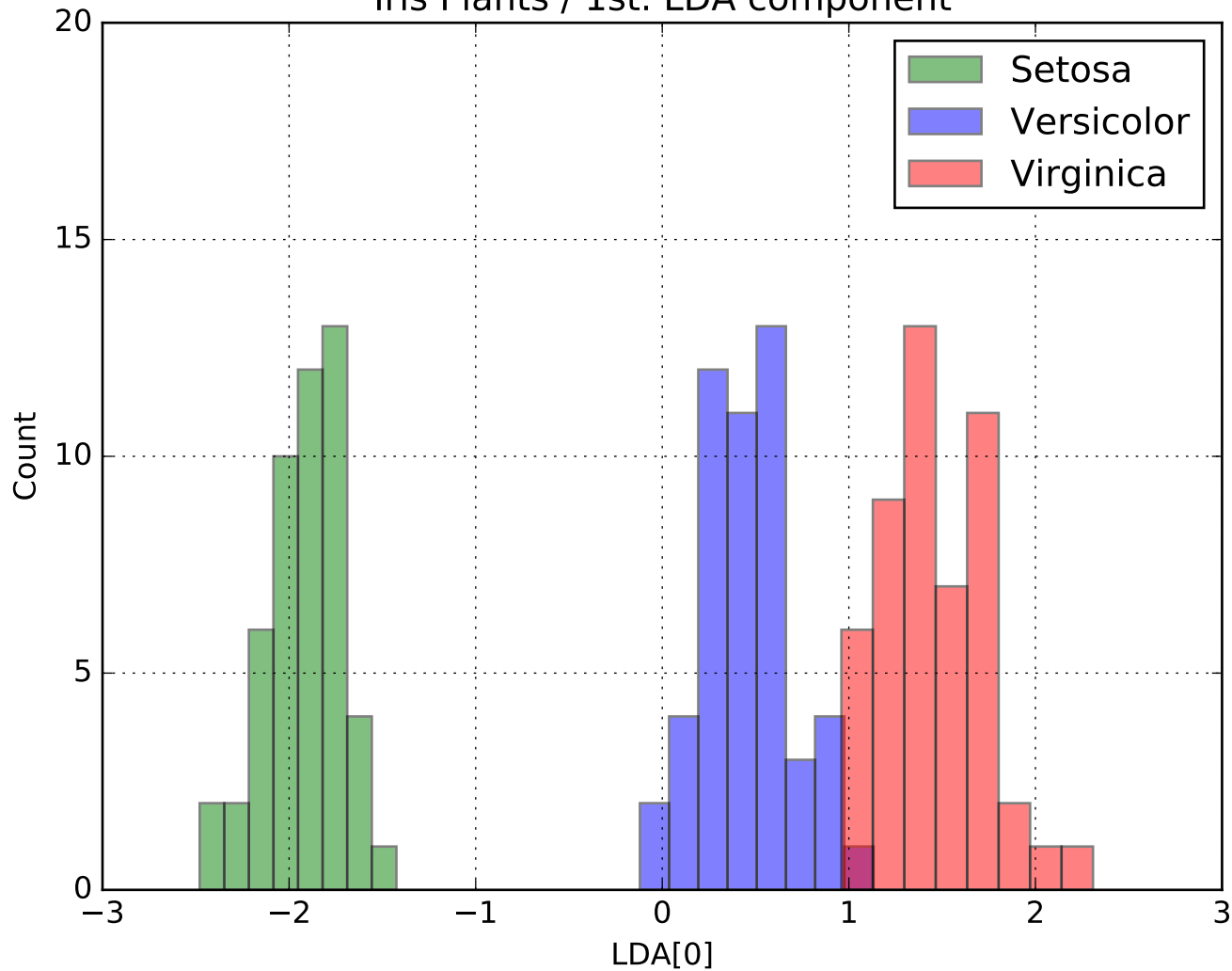
Iris Plants / 1st. LDA component
